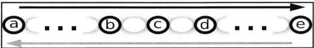
Figure 1 Logistics chain
